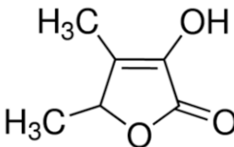
Figure 6. Structure of Fenugreek Lactone.
