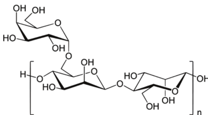
Figure 5. Galactomannan Structure.
